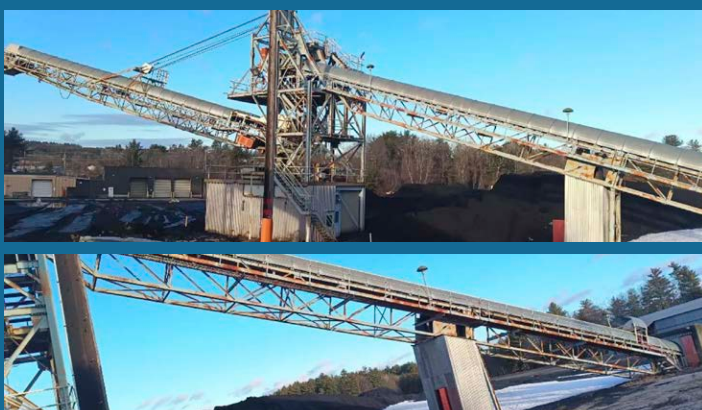
Boom Conveyor , with GE 8000 Line Motor Control, (Lot 6502)
